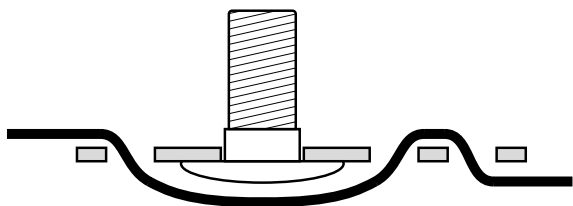
Fig. 10. Bolt attachment to the strap
